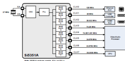
Using the Si5351A to Replace Multiple Crystals, Crystal Oscillators, and PLLs
